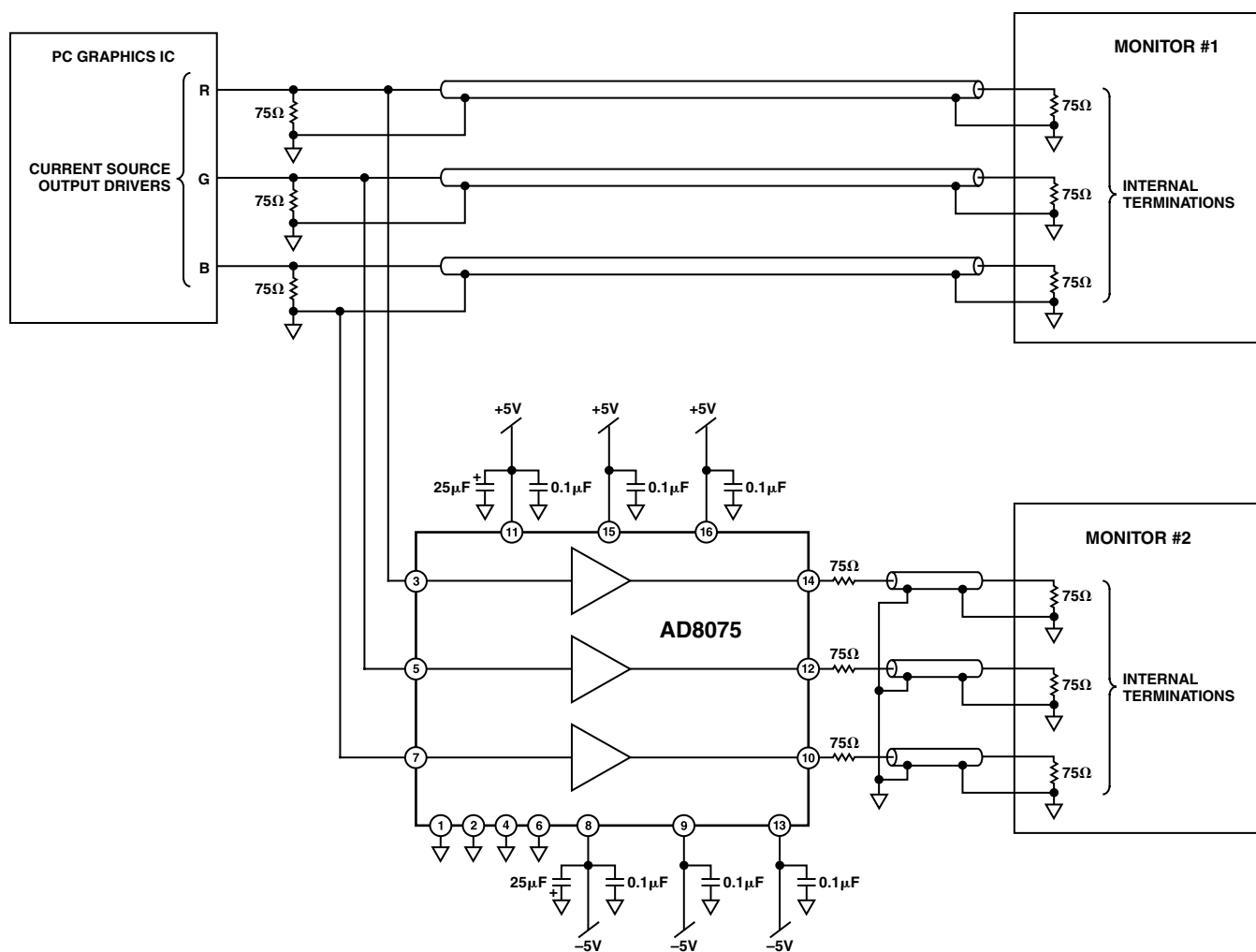
Figure 3. Buffer
