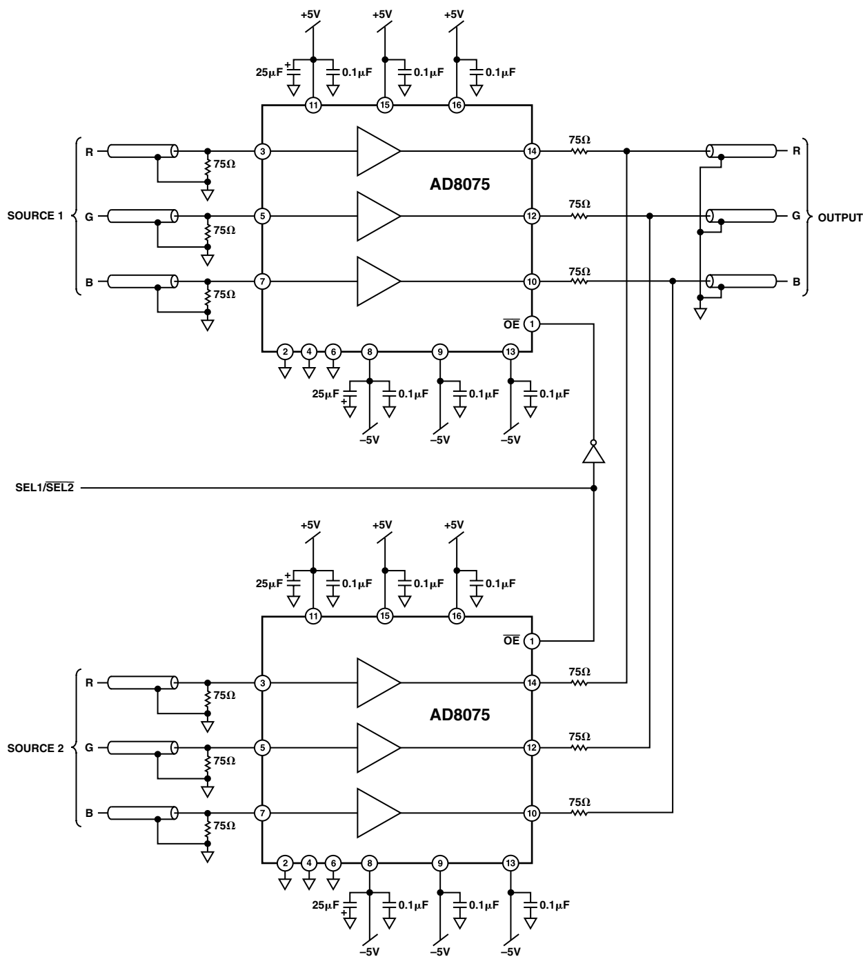
Figure 4. Mux
