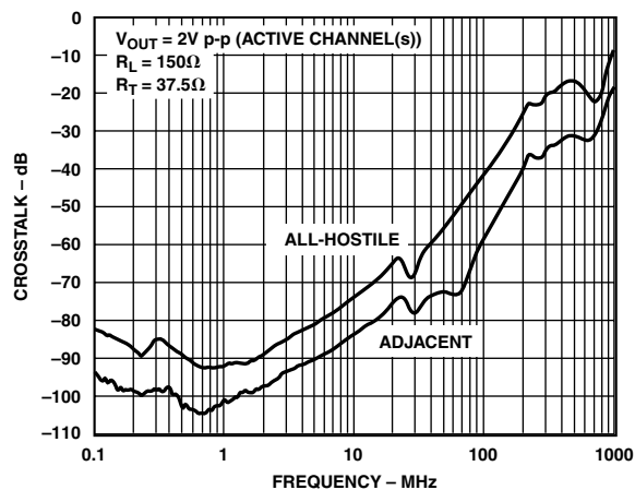
TPC 9. AD8075 Crosstalk vs. Frequency (All Hostile and Adjacent R_L = 150\text{ }\Omega )
