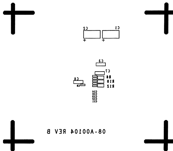
Figure 9. Silkscreen Bottom
