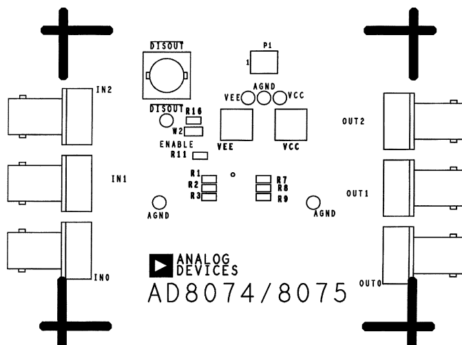
Figure 8. Silkscreen Top
