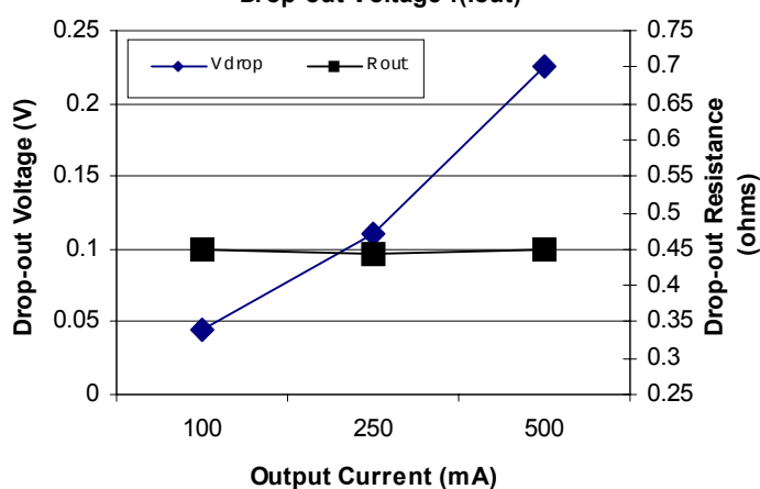
Drop-out Voltage f(lout)
