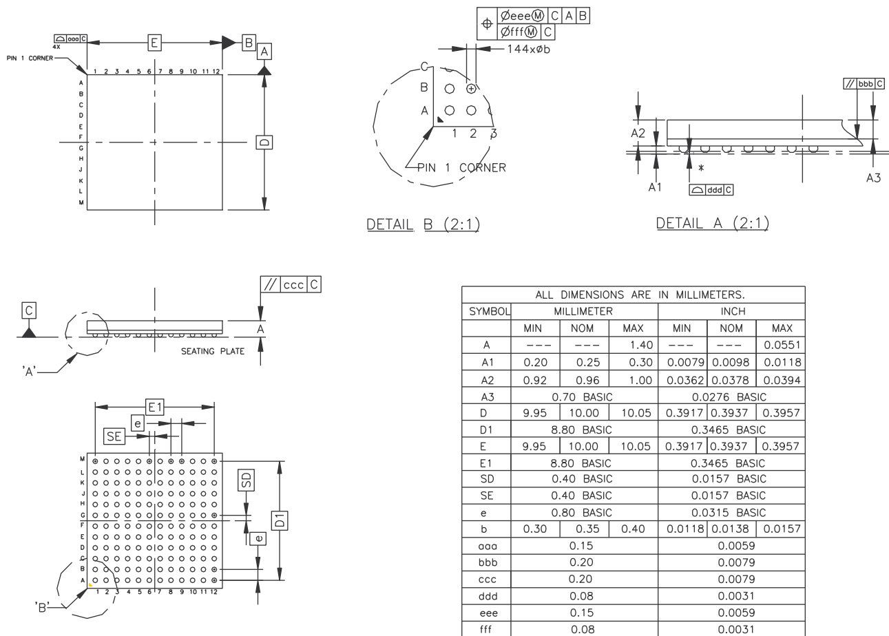
Figure 12-1. 144-ball BGA Package Drawing
