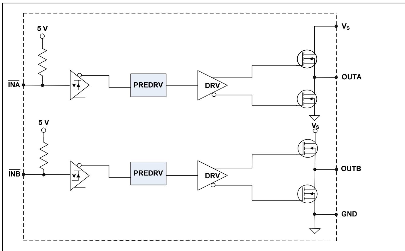
Functional Block Diagram: AUIRS4426
