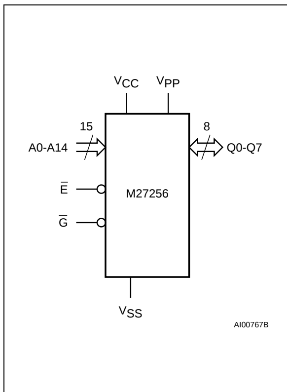
Figure 1. Logic Diagram
