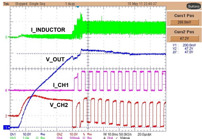
FIGURE 13. START-UP WITH PHASE SHIFT ( V_{IN} : 19V, I_{CH} : 120mA, LEDs: 4P18S, f_{DIM} : 200Hz)
