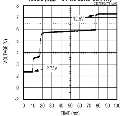
CHARGE-PUMP STARTUP EXITING SLEEP MODE ( V_{DD} = 8V NO LOAD ON PK+)
