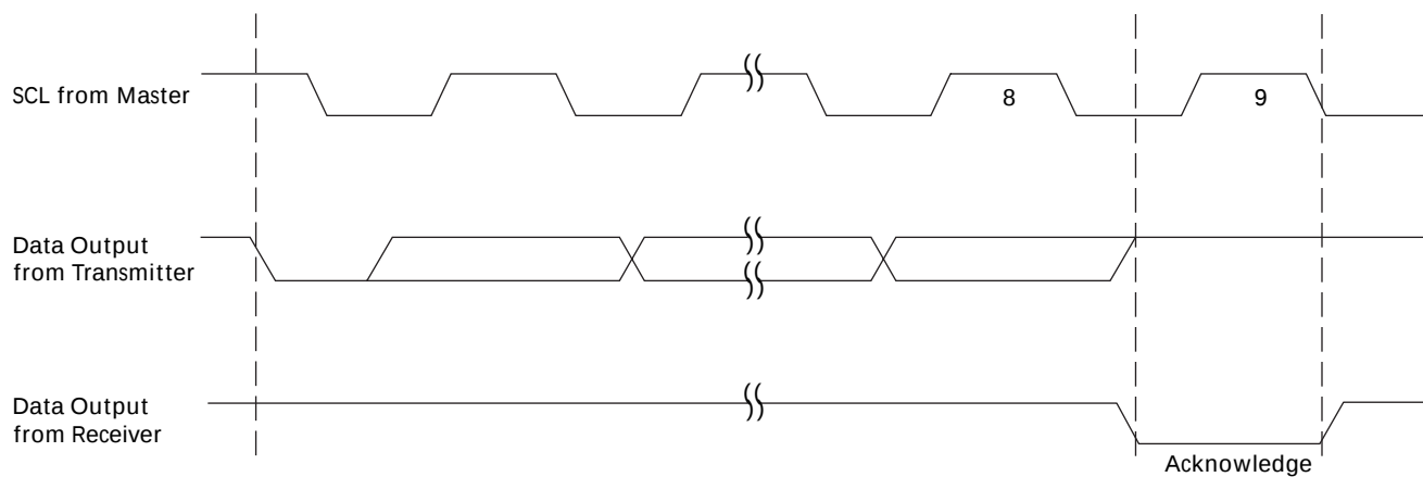
Figure 6: Acknowledge Response From Receiver
