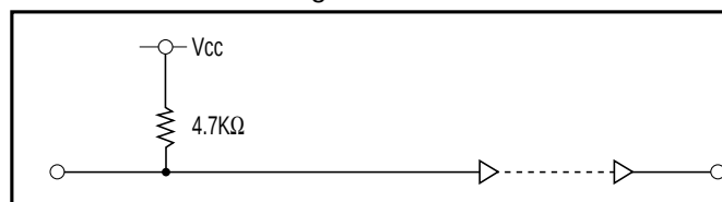
Buffer circuit detailed diagram
