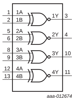
Fig 1. Functional diagram
