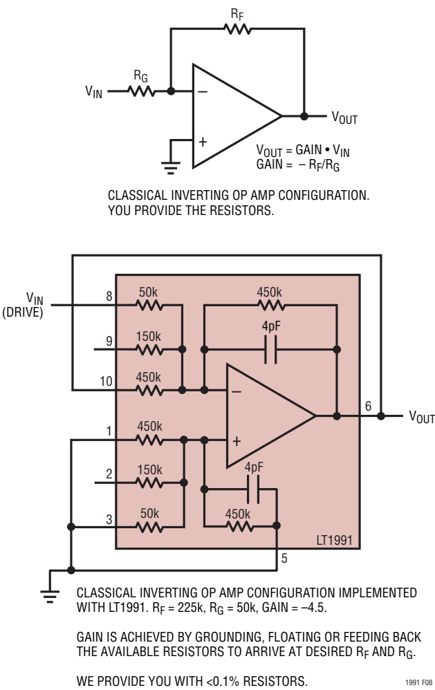
Figure 8. The LT1991 as a Classical Inverting Op Amp. Note the Circuit Is Identical to the Noninverting Amplifier, Except that V_{IN} and Ground Have Been Swapped
