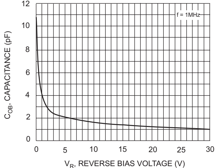
Fig. 4 Output Capacitance
