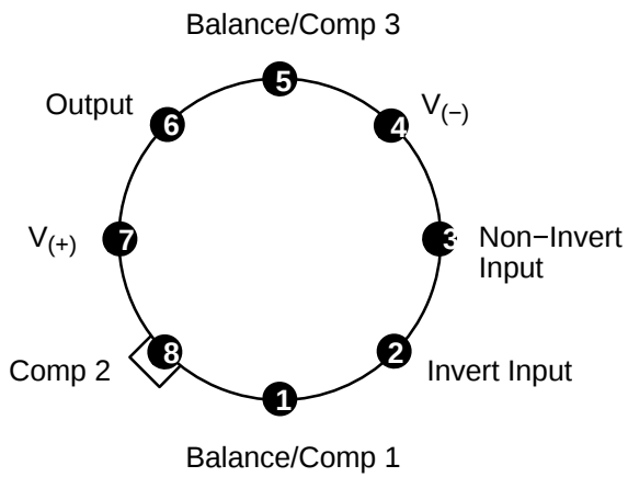
NTE918 (Top View)
