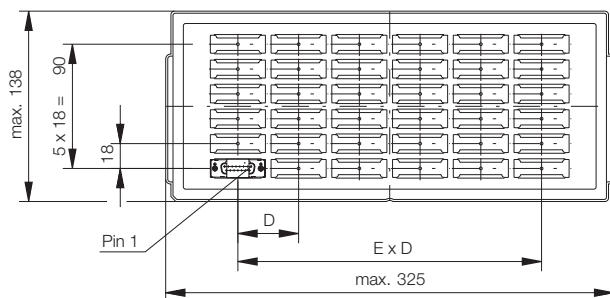
Tray packaging (15pin version pictured)
