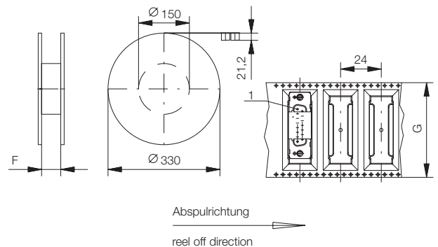
Tape and reel packaging (15pin version pictured)
