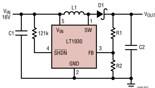
Figure 7. Keeping \overline{SHDN} Below 10V
