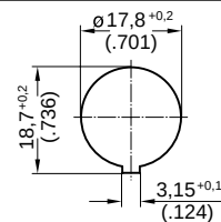
Panel cutout
