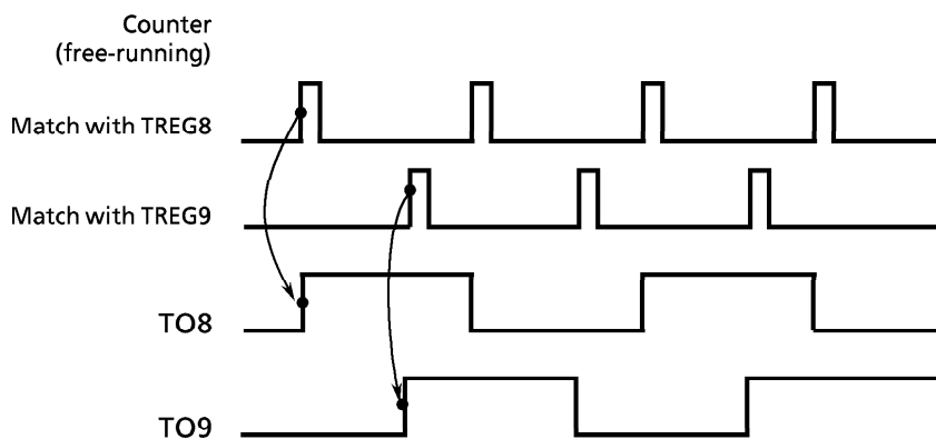
Figure 3.8 (11) Phase Output
