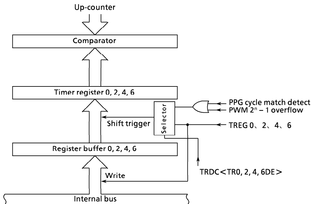
Figure 3.7 (4) Configuration of Timer Registers 0, 2, 4, 6
