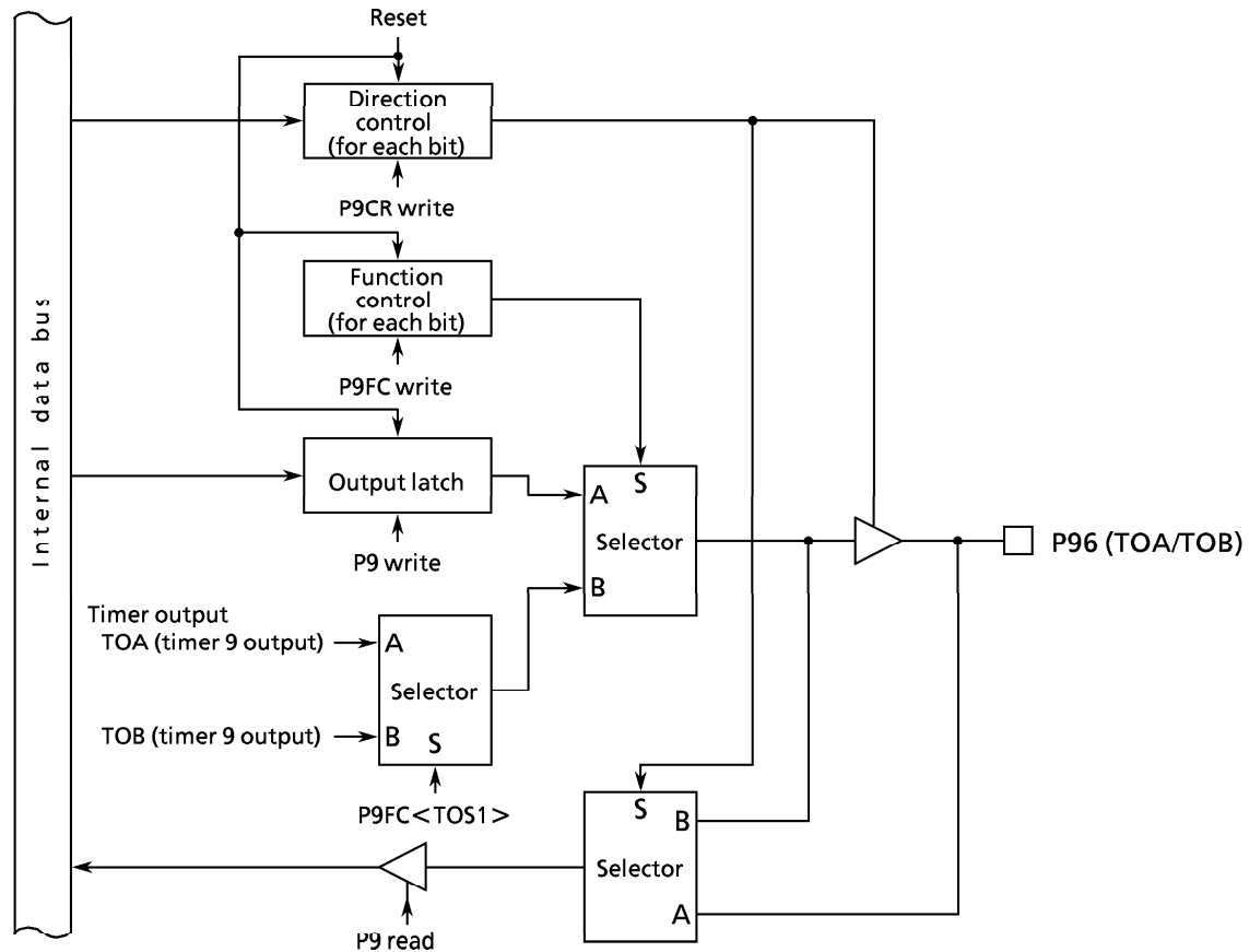
Figure 3.5 (32) Port 9 (P96)
