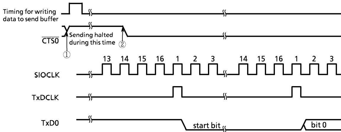
Figure 3.9 (4) Handshake Function
