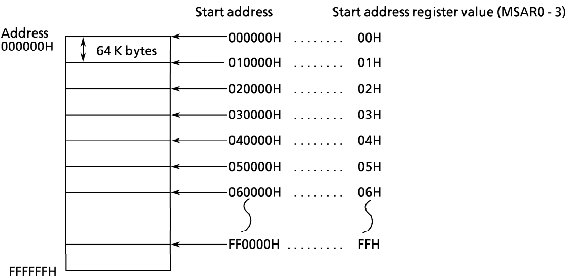
Figure 3.6 (2) Relationship Between Start Address and Start Address Register Value
