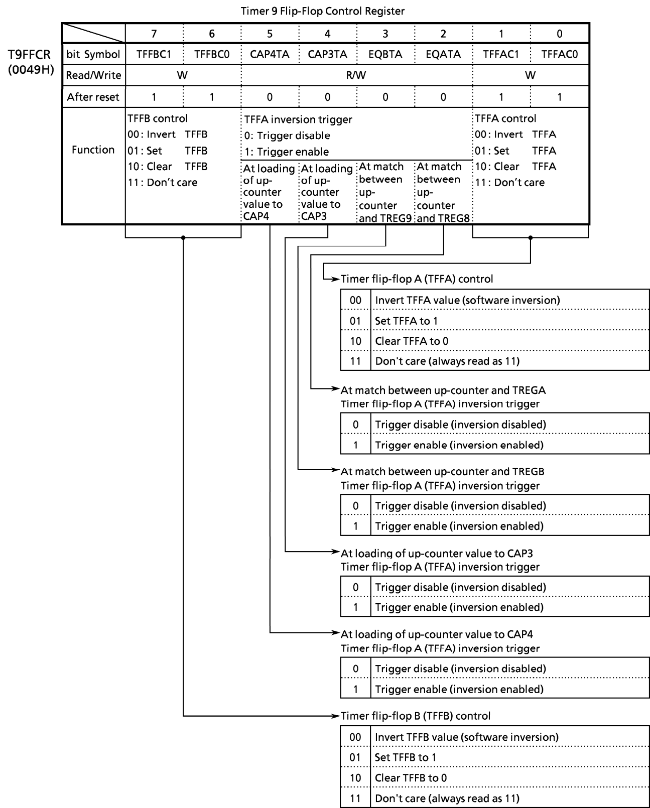
Figure 3.8 (2)-5 16-Bit Timer/Event Counter Related Register
