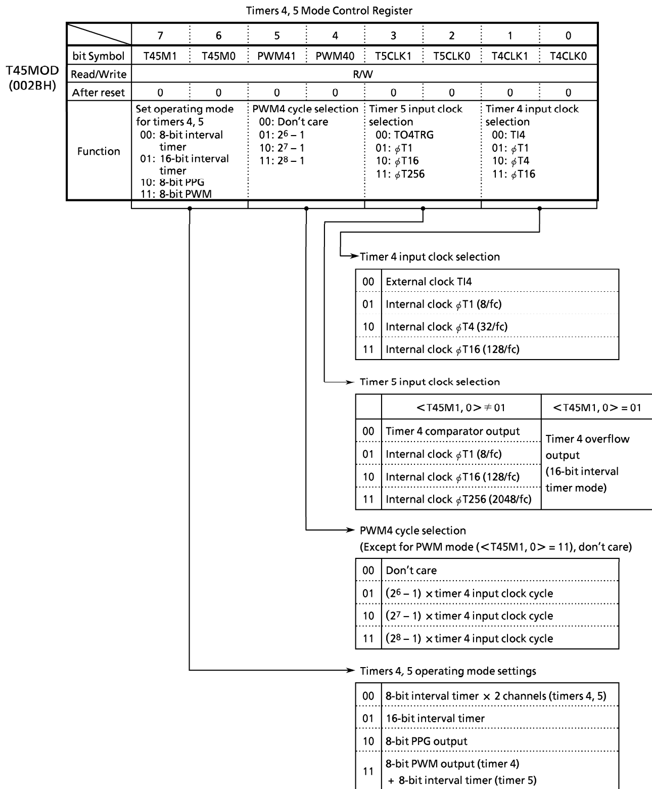
Figure 3.7 (2)-5 8-Bit Timer Related Register
