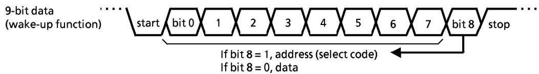
Figure 3.9 (6) Data Formats
