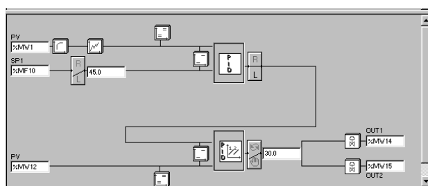
Cascaded loop
