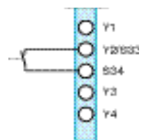
Manual reset without start button monitoring
