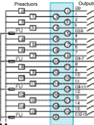
FU: fuse to be rated according to load
