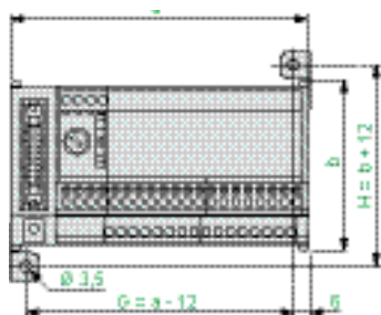
Fixing centers for sub-bases using mounting kit ABE 7ACC01
