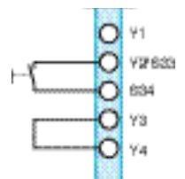
Manual reset with start button monitoring
