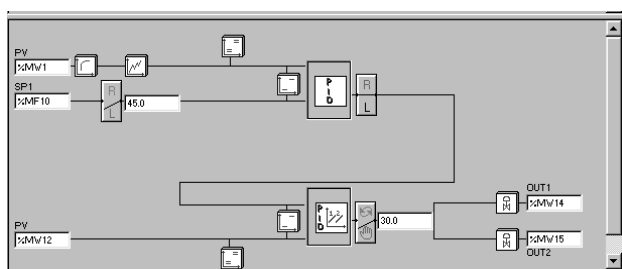
Cascaded loop
