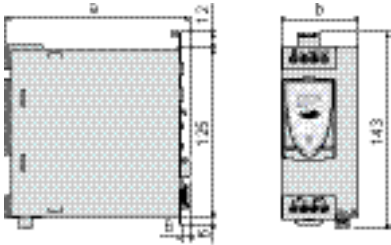
ABL 8RPS24030
