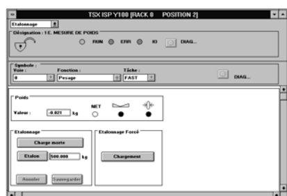
Weigher calibration
