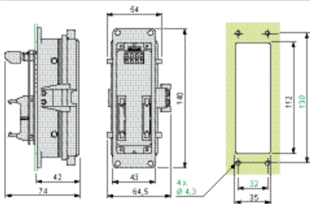
ABE 7ACC84
