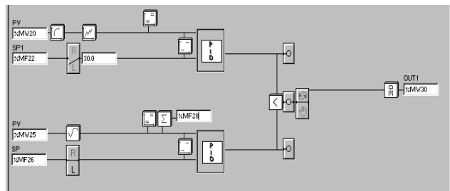
Autoselective loop
