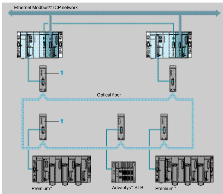
1 OZD FIP G3 fiber-optic transmitter (see page 5/85).
