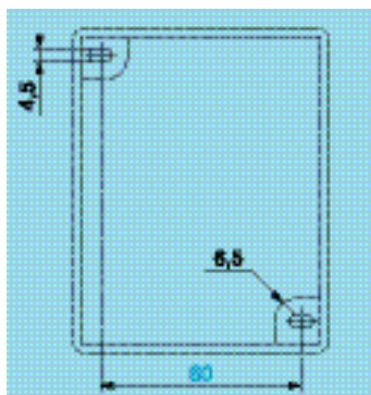
Mouting zener barrier box SM1 PY52
