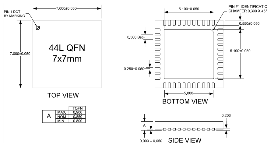
Figure 2. 44-pin TQFN Package Dimensions
