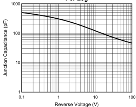
Fig. 6 – Typical Junction Capacitance Per Leg
