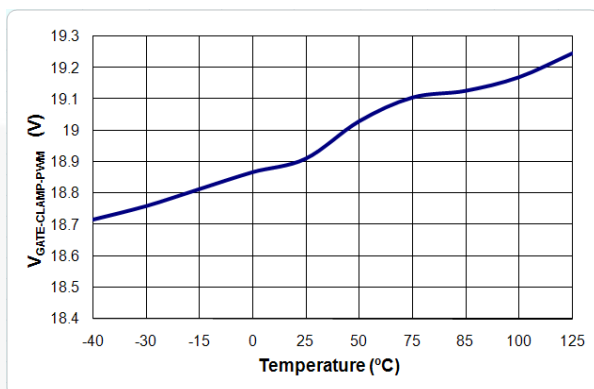
Figure 20. V_{\text{GATE-CLAMP-PWM}} vs. Temperature
