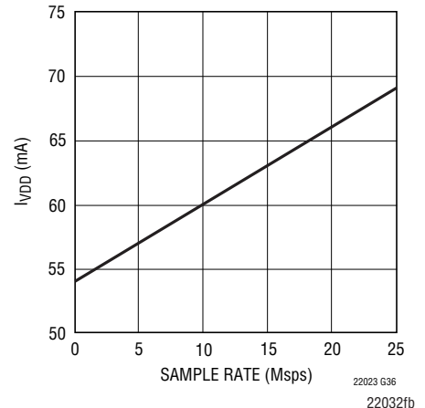
LTC2203: I_{VDD} vs Sample Rate, 5MHz Sine Wave, -1\text{dBFS}
