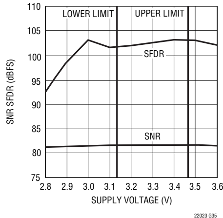
LTC2203: SNR and SFDR vs Supply Voltage ( V_{DD} ), f_{IN} = 5\text{MHz}
