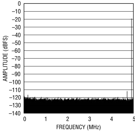
LTC2203: 128K Point FFT, f_{IN} = 5.1\text{MHz} , -20\text{dBFS} , \text{PGA} = 0 , Internal Dither "On"
