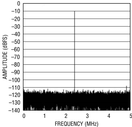
LTC2202: 32K Point FFT, f_{IN} = 12.4\text{MHz} , -10\text{dBFS} , \text{PGA} = 0
