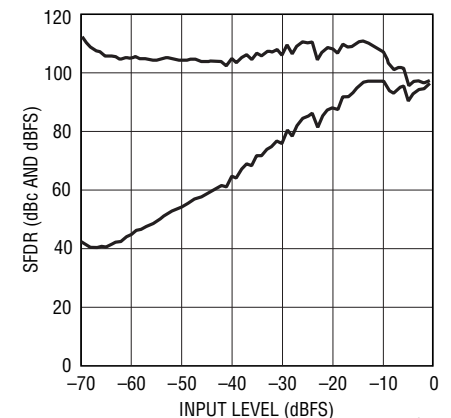
LTC2202: SFDR vs Input Level, f_{IN} = 12.4\text{MHz} , \text{PGA} = 0 , Dither "Off"
