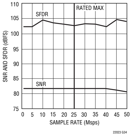
LTC2203: SNR and SFDR vs Sample Rate
