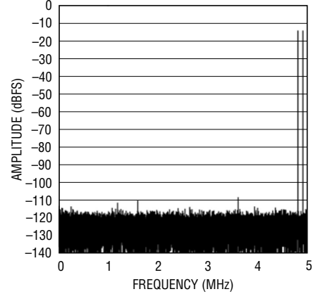
LTC2202: 32K Point 2-Tone FFT, f_{IN} = 5.1\text{MHz} and 15.2\text{MHz} , -15\text{dBFS} , \text{PGA} = 0
