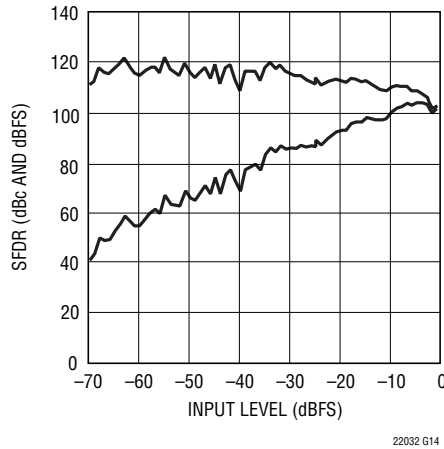
LTC2203: SFDR vs Input Level, f_{IN} = 5\text{MHz} , \text{PGA} = 0 , Dither "On"
