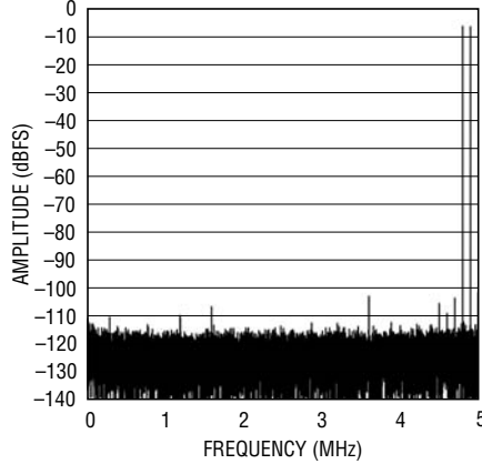
LTC2202: 32K Point 2-Tone FFT, f_{IN} = 5.1\text{MHz} and 15.2\text{MHz} , -7\text{dBFS} , \text{PGA} = 0
