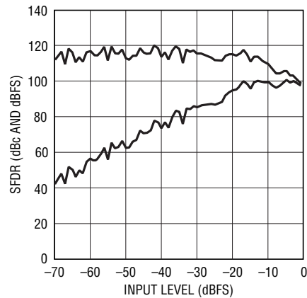
LTC2202: SFDR vs Input Level, f_{IN} = 5\text{MHz} , \text{PGA} = 0 , Dither "On"
