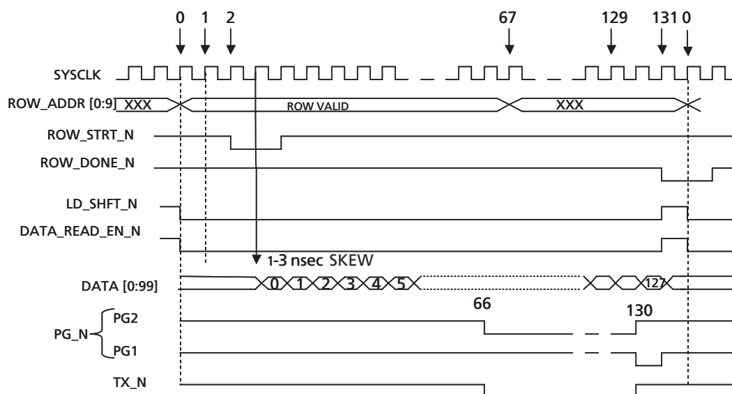
Figure 7: Timing Diagram for One Row
