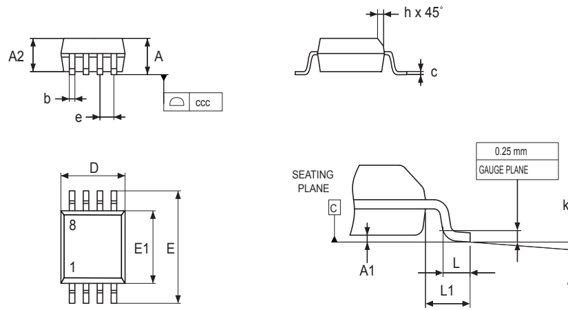
Figure 78. SO8N – Outline
