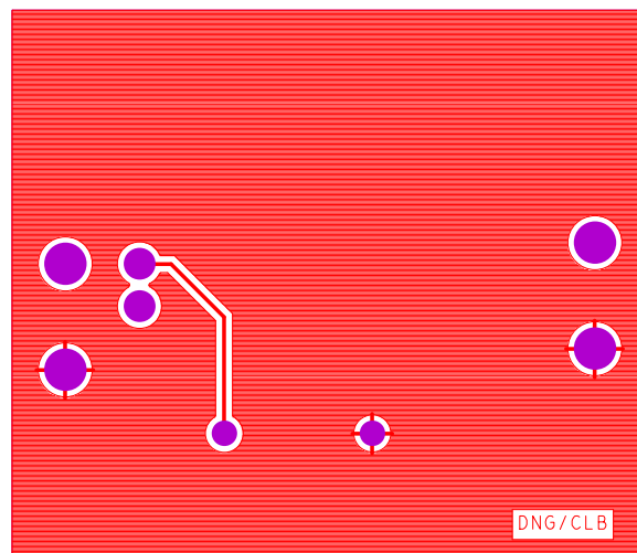
FIGURE 3. BOTTOM LAYER
