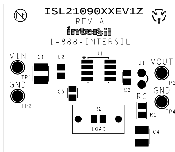
FIGURE 4. ASSEMBLY DRAWING
