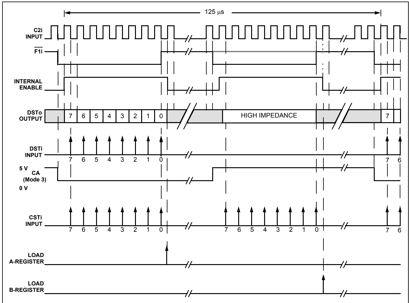
Figure 9a - Timing Diagram - 125 \mu\text{s} Frame Period
