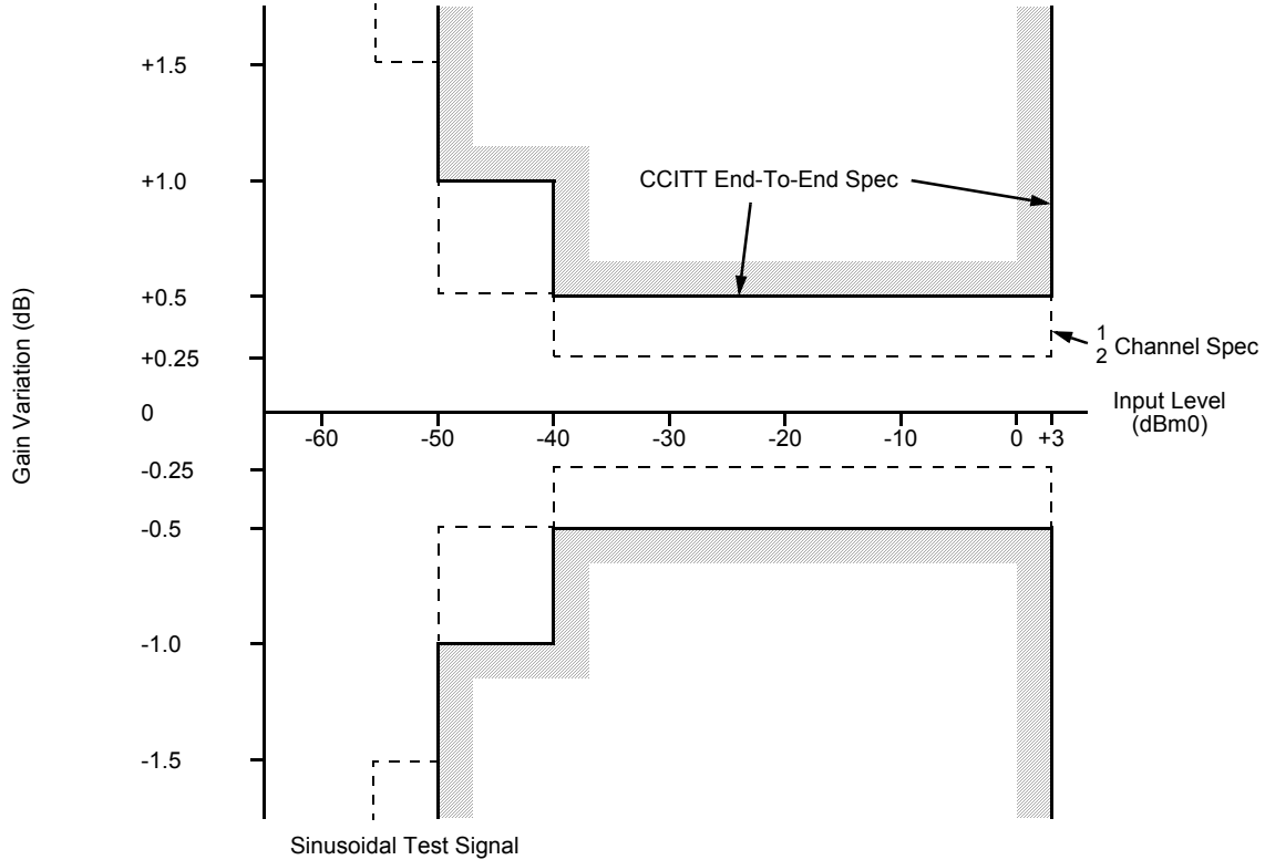
Figure 12 - Variation of Gain With Input Level
