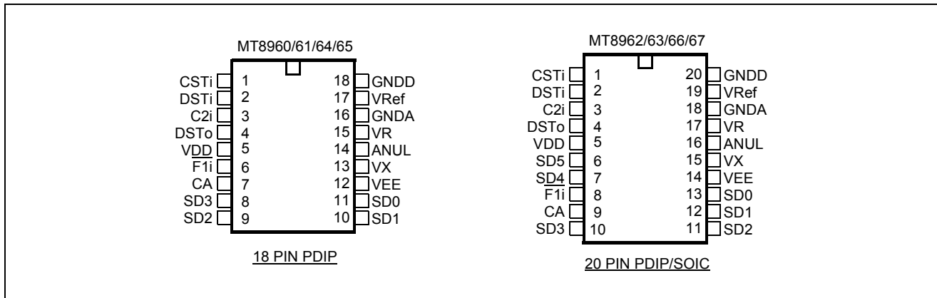
Figure 2 - Pin Connections
