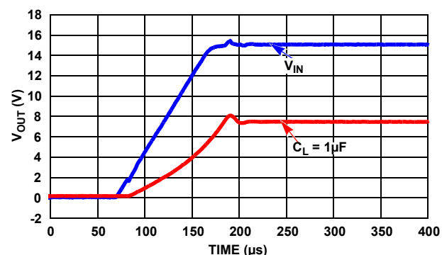
FIGURE 61. TURN-ON TIME WITH 1μF
