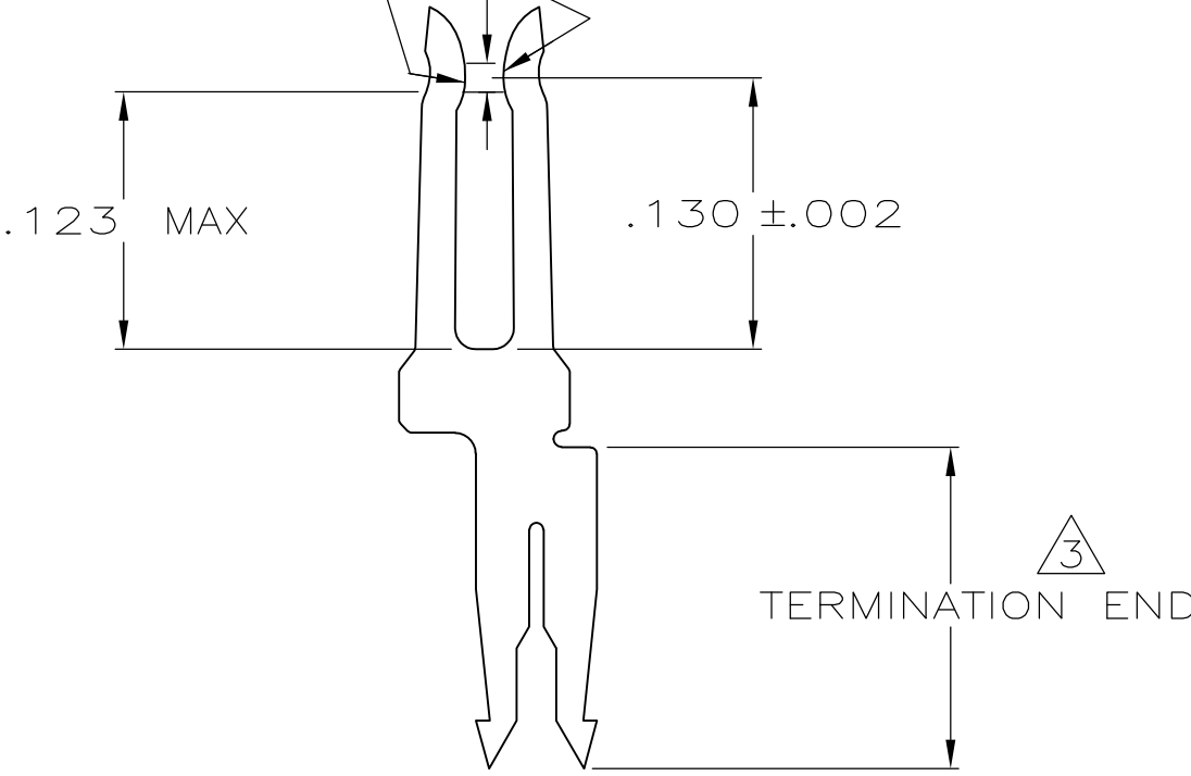
DETAIL Z SCALE 10:1 TYPICAL
