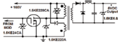
TVSD in SMPS Output Protection
