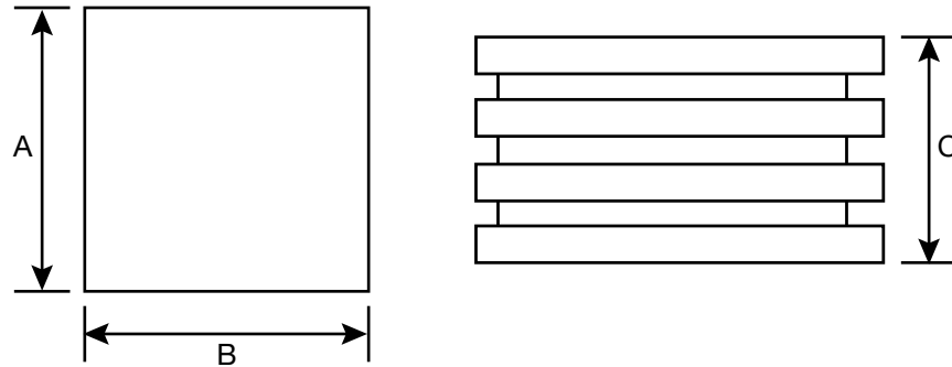
WFC0.5, WFC1, WFC1.5, WFC A, WFC B, WFC C SERIES DIMENSIONS
