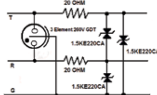
GDT & TVSD In Telephone Line Protection
