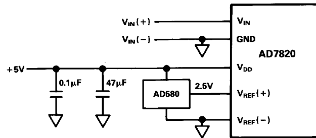
Figure 7b. External Reference 2.5V Full-Scale
