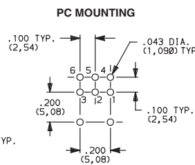
T201MH9ABE Horizontal Actuation DPDT
