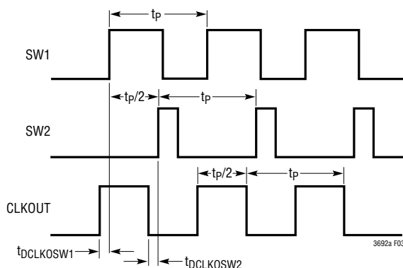
Figure 3. Timing Diagram R_{T/SYNC} = 28.0k , t_p = 1\mu s , V_{DI} = 0V
