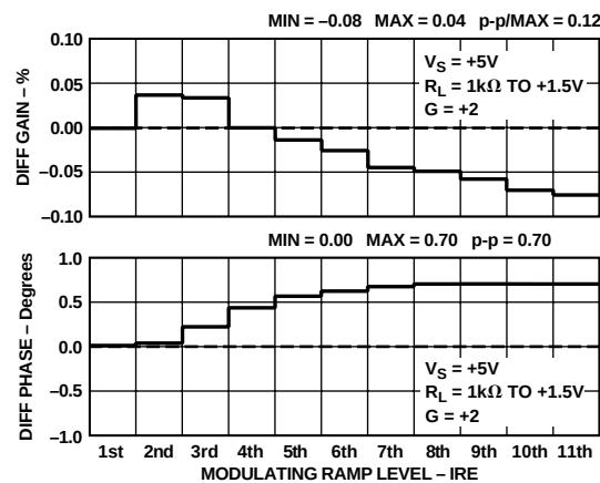
Figure 14. Differential Gain and Phase, V_S = +5\text{ V}
