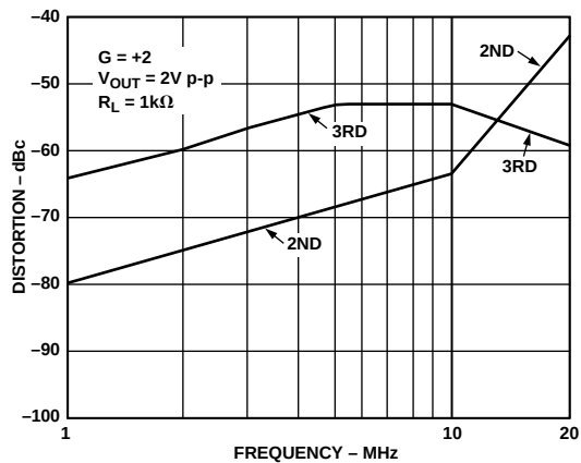
Figure 10. Distortion vs. Frequency; V_S = \pm 5\text{ V}
