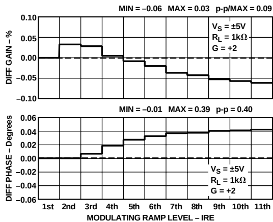
Figure 11. Differential Gain and Phase, V_S = \pm 5\text{ V}
