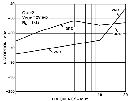
Figure 13. Distortion vs. Frequency V_S = +5\text{ V}
