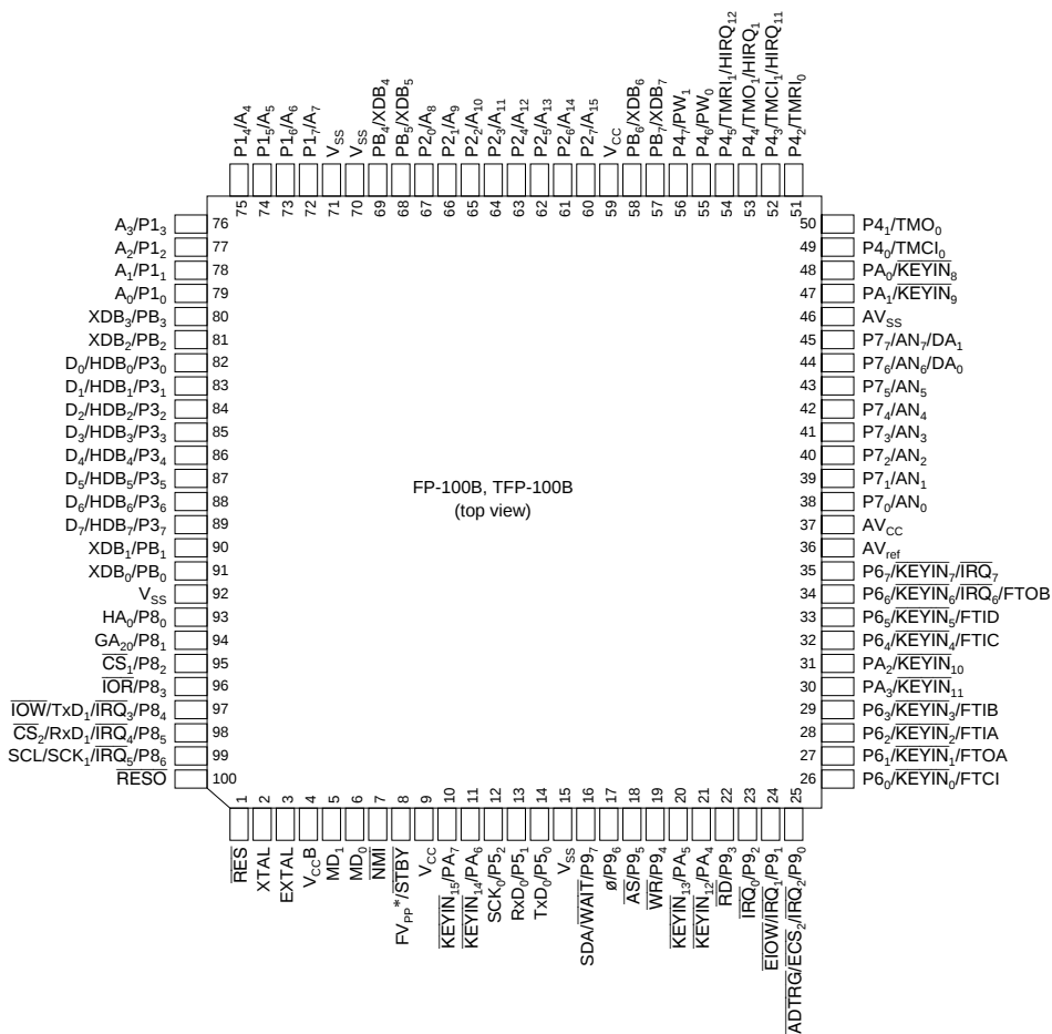
Figure 1.2 Pin Arrangement (FP-100B, TFP-100B, Top View)
