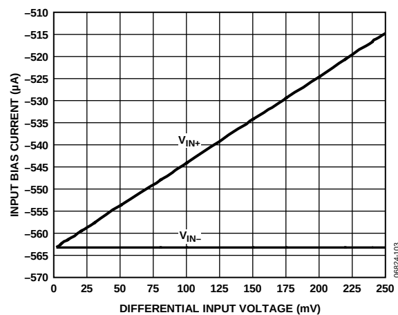
Figure 9. Input Bias Current vs. Differential Input Voltage, V_{CM} = 0 V
