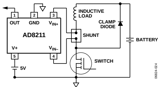
Figure 25. Low-Side Switch
