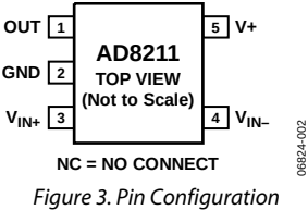
Figure 3. Pin Configuration
