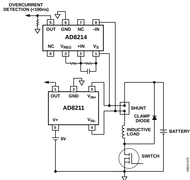
Figure 26. Battery-Referenced Shunt Resistor
