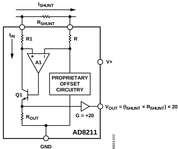
Figure 23. Simplified Schematic
