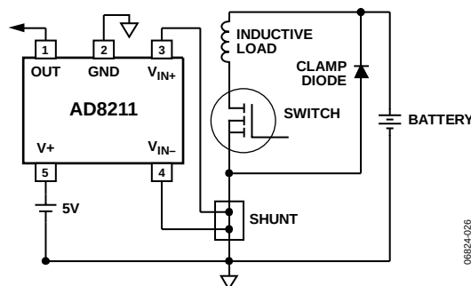
Figure 27. Ground-Referenced Shunt Resistor
