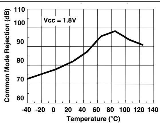
Figure 8. Common mode rejection vs. temperature at Vcc = 1.8 V
