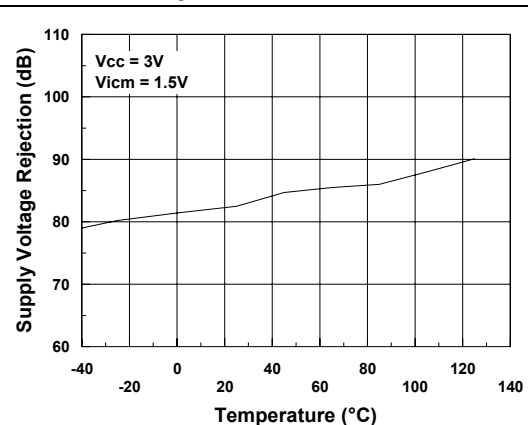
Figure 12. Supply voltage rejection vs. temperature at Vcc = 3 V
