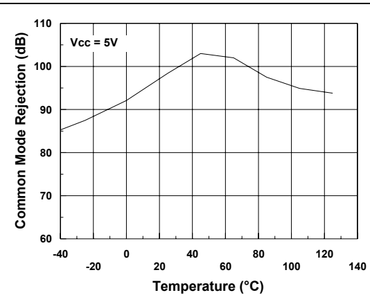
Figure 10. Common mode rejection vs. temperature at Vcc = 5 V
