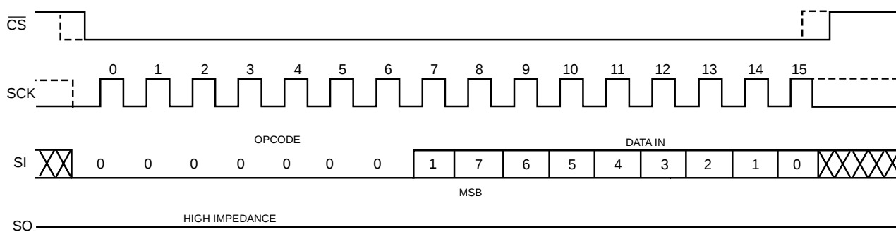
Figure 8. WRSR Timing
