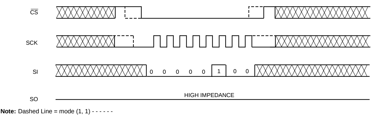
Figure 5. WRDI Timing
