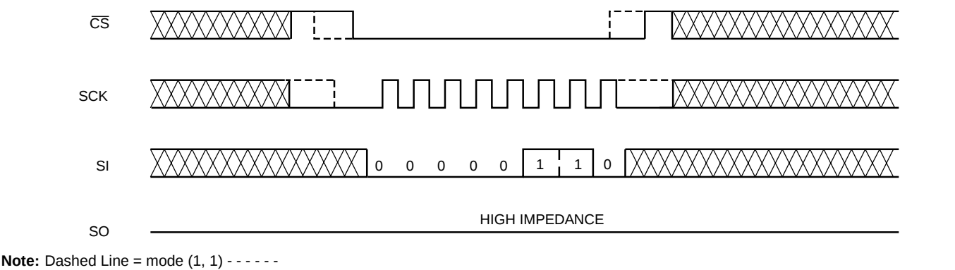
Figure 4. WREN Timing
