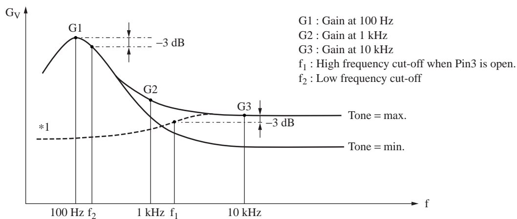
Fig. Frequency response of AN5270
