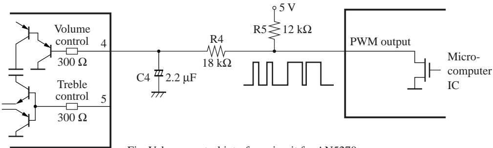
Fig. Volume control interface circuit for AN5270
