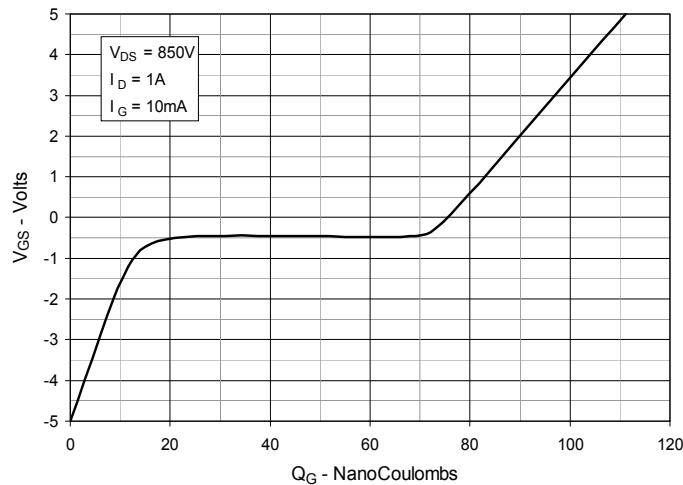
Fig. 15. Gate Charge
