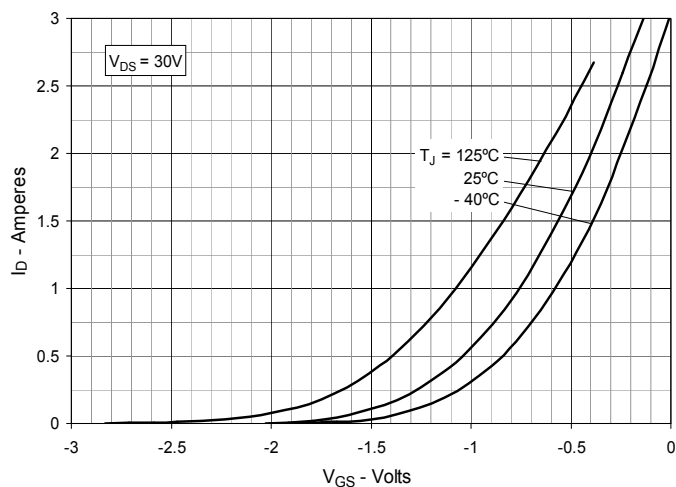
Fig. 10. Input Admittance
