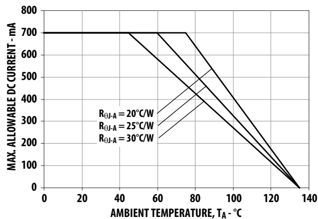
Figure 13 Maximum Forward Current vs. Ambient Temperature. Derated based on T_{J\text{MAX}} = 125^{\circ}\text{C} , R_{\theta J-A} = 20^{\circ}\text{C/W} , 25^{\circ}\text{C/W} , and 30^{\circ}\text{C/W} .
