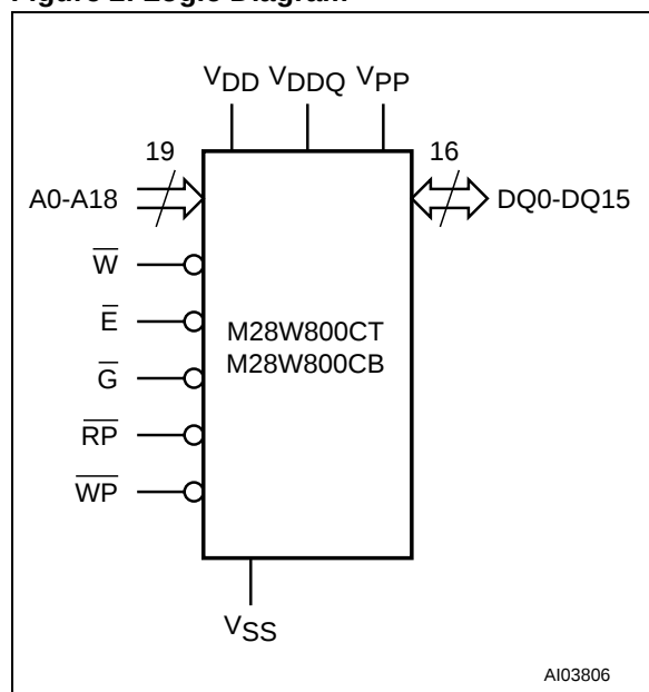
Figure 2. Logic Diagram
