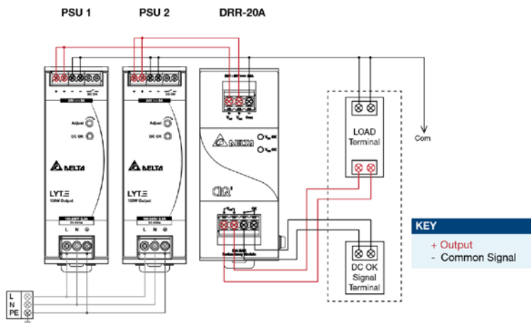
Fig. 3 Redundancy Operation Connection Diagram
