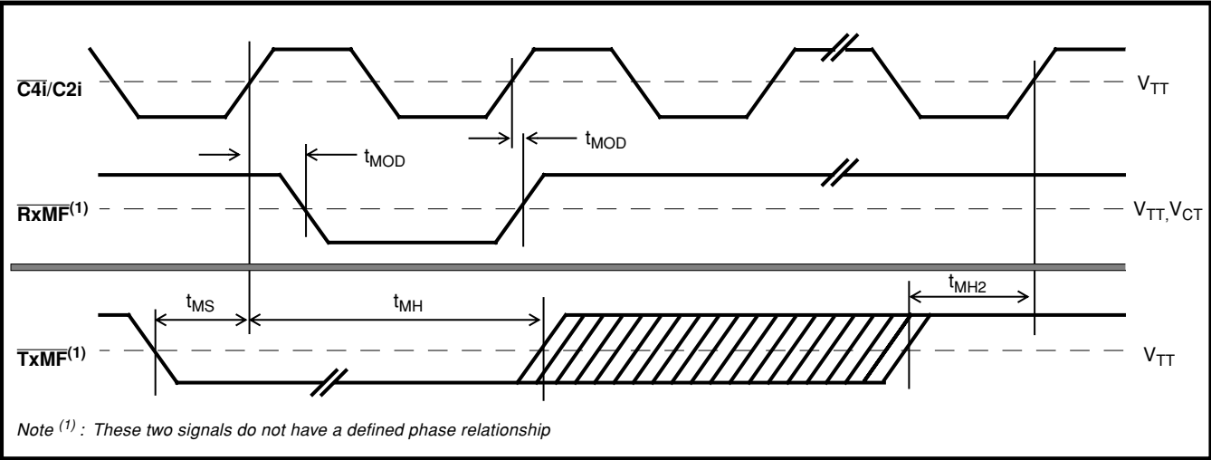
Figure 25 - Multiframe Timing Diagram (C4i/C2i = 2.048 MHz)
