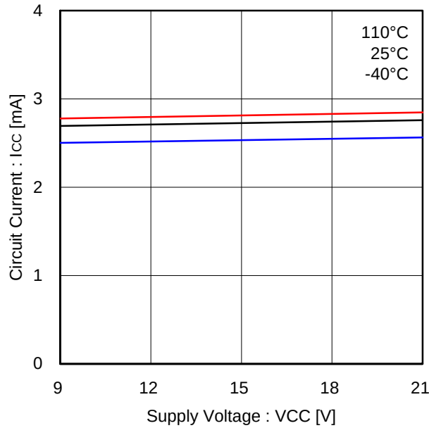
Figure 9. Circuit current
