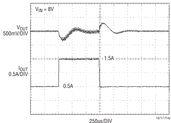
Figure 14a. Load Transient Response for the Circuit in Figure 9
