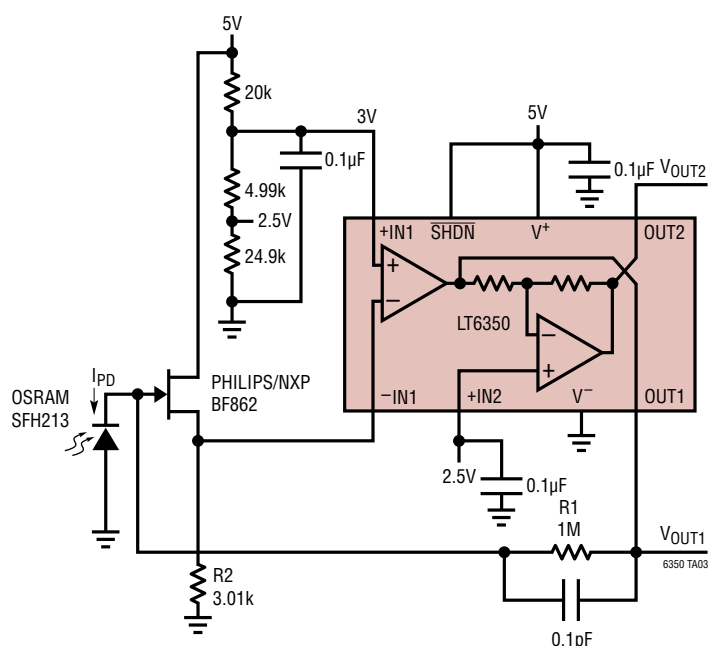
Low Noise, Low Power 1M \Omega Single Supply Photodiode Transimpedance Amplifier
