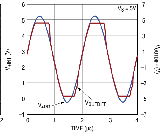
Overdrive Recovery
