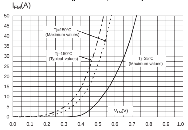
Figure 6: Forward voltage drop versus forward current (per diode, low level)
