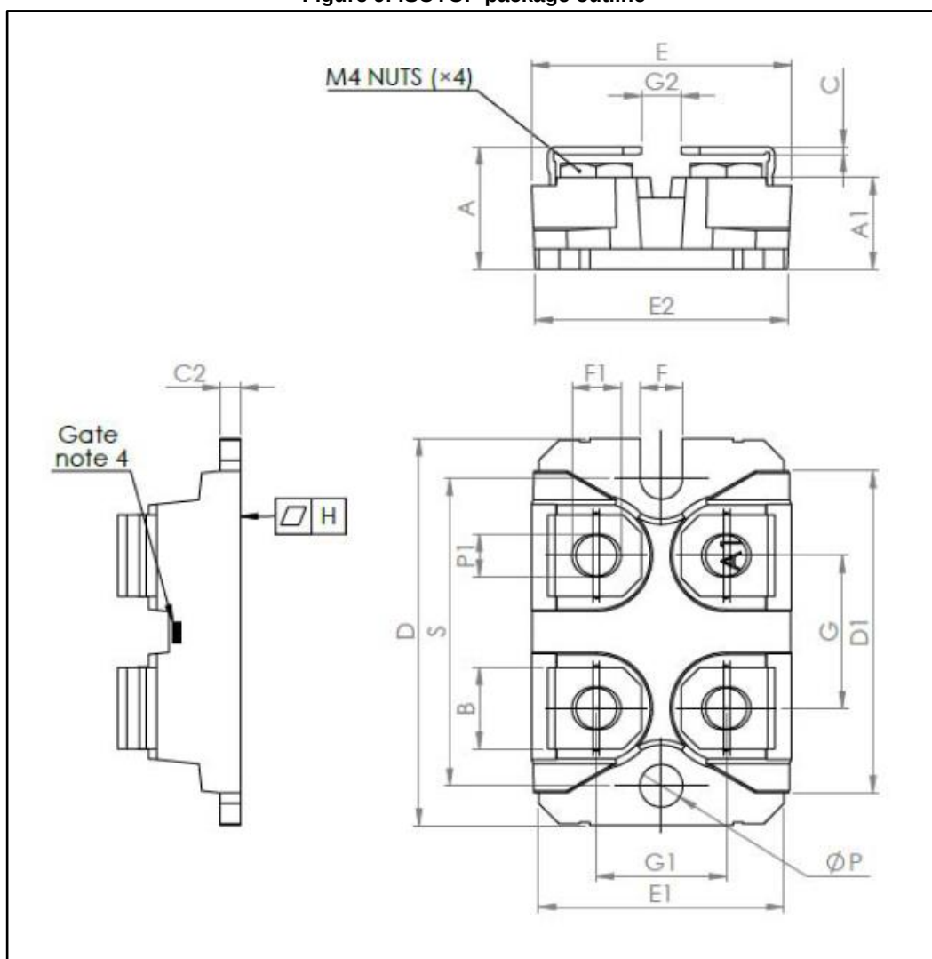
Figure 9: ISOTOP package outline
