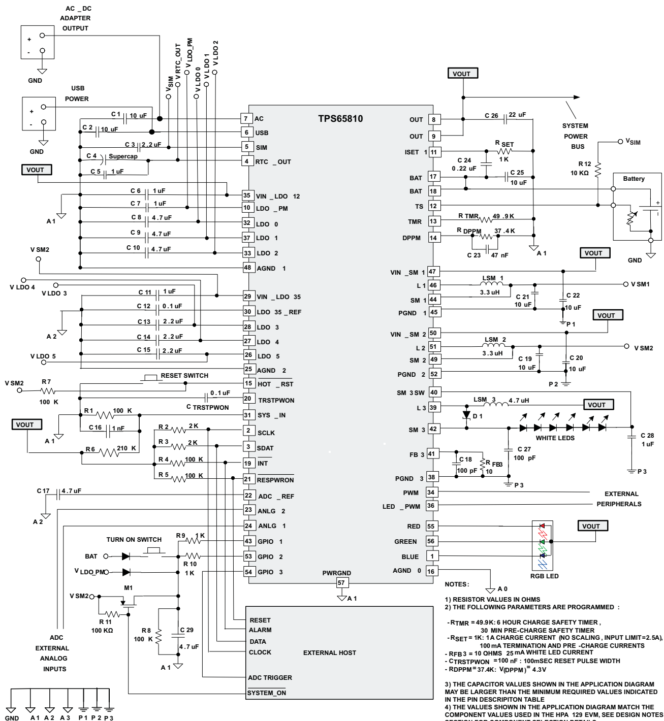
Figure 51. TPS65810 Application Diagram, Recommended External Components
