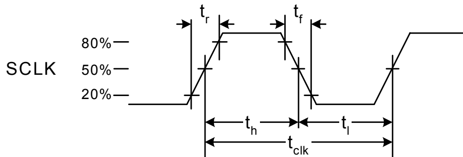
Figure 1. SCLK Timing Diagram
