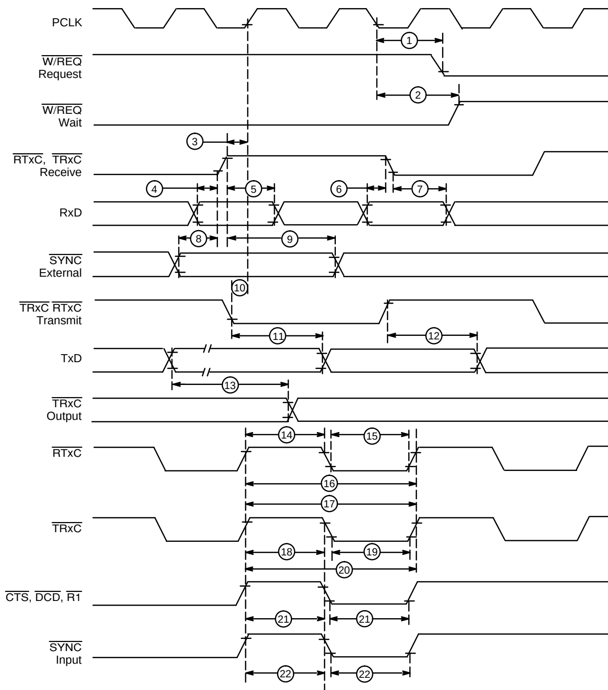
Figure 19. General Timing
